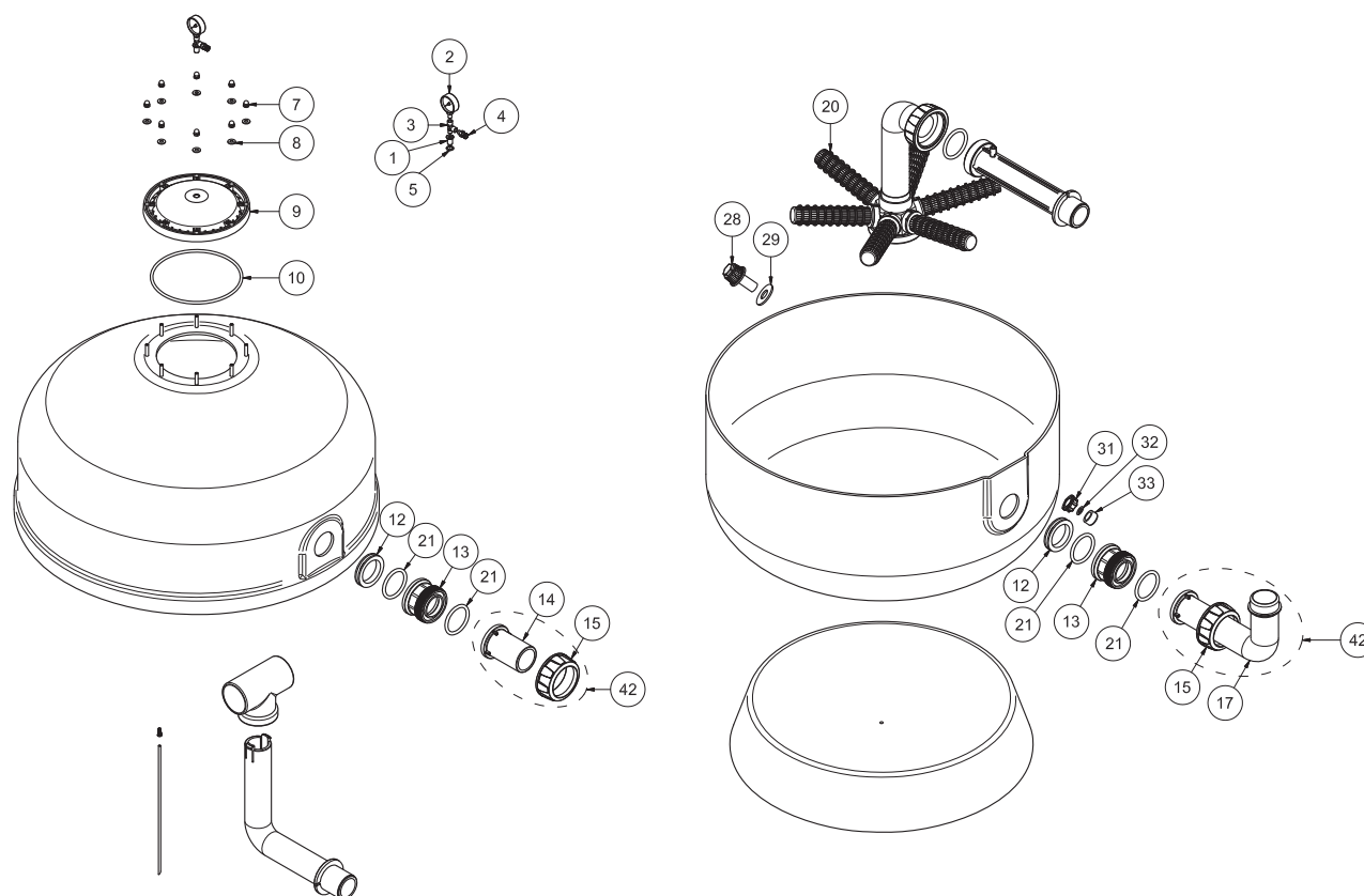
Esplso AQUAGLASS/ AQUAGLASS Exploded Drawing
